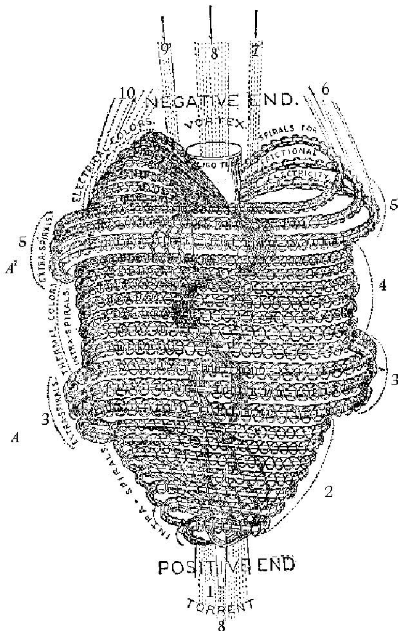
Fig. 135. The general Form of an Atom, including the spirals and 1st Spinillae, together with influx and efflux ethers, represented by dots, which pass through these spinillae. The 2nd and 3rd spirillae with their still finer ethers are not shown.
